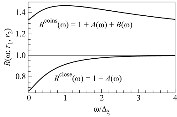
Fig.1. The LDOS correlation function vs. \omega/\Delta_\xi : at coincident points, R^{\text{coins}}(\omega) , and at k_F^{-1} \ll |\mathbf{r}_1 - \mathbf{r}_2| \ll \xi , R^{\text{close}}(\omega)
