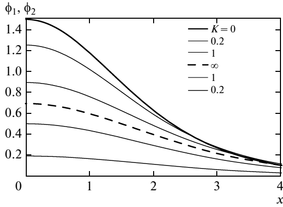
Fig. 2. Numerical solutions of Eqs. (34a) and (34b) in 1D geometry ( d = 1 ) for various values of the replica-mixing parameter K . For K = 0 , \phi_1(x) = 0 , and \phi_2(x) = \phi_{\text{inst}}^{(1)}(x) (the upper thick curve). Solutions for intermediate values ( K = 0.2 and K = 1 ) are shown by the thin solid curves. In the limit K \rightarrow \infty , \phi_1(x) and \phi_2(x) approach the asymptote \phi_{\text{inst}}^{(-1)}(x) (the thick dashed curve).
