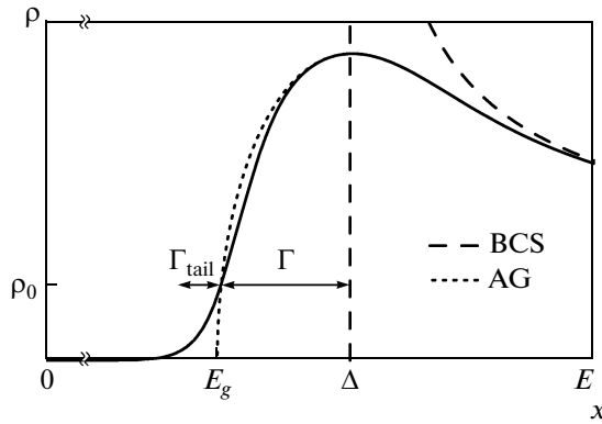
Fig. 1. Schematic view of the average DOS in a dirty superconductor (solid curve). Broadening of the BCS peak (dashed curve) is mainly described by the semiclassical approximation (dotted curve), with the full DOS containing a significant tail of subgap states.
